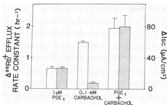
Figure 7. Comparison of ^{86}\text{Rb}^+ efflux across the basolateral membrane and I_{\text{sc}} . Results are expressed as mean \pm SE of 6–8 monolayers. Average changes in rate constant of ^{86}\text{Rb}^+ efflux per hour in the first 10 min after the addition of carbachol and/or \text{PGE}_1 are expressed as clear bars, while changes in I_{\text{sc}} represent changes in the rate of \text{Cl}^- secretion, and are shown as solid bars. Basal rate constants for ^{86}\text{Rb}^+ efflux in the first 20 min were 0.48 \pm 0.04 , 0.56 \pm 0.06 , and 0.43 \pm 0.02 in \text{PGE}_1 , carbachol, and \text{PGE}_1 + carbachol groups, respectively, while basal I_{\text{sc}} were 3 \pm 1 , 4 \pm 2 , and 1 \pm 1 \mu\text{A}/\text{cm}^2 , respectively. These basal values were subtracted from the observed responses to obtain the results shown in the figure.
