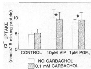
Figure 6. Lack of effect of carbachol on \text{PGE}_1 or VIP-stimulated ^{36}\text{Cl}^- uptake across the apical membrane. Conditions for uptake studies are as described in Fig. 5. Results are mean \pm SE of \text{Cl}^- uptake from five monolayers in each group. Results at 5 min, when carbachol's action was at its peak, are shown. Asterisks indicate P < 0.05 by unpaired t test as compared with control without VIP or \text{PGE}_1 . Carbachol does not alter the increased uptake stimulated by \text{PGE}_1 or VIP.
