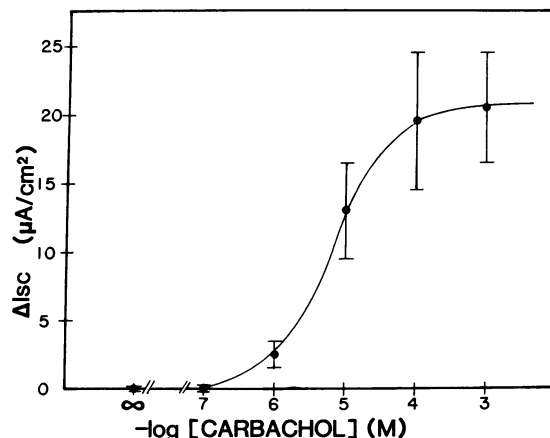
Figure 2. Graded dose effect of carbachol on the changes in I_{sc} . Carbachol was added to the serosal reservoir in concentrations shown. The peak I_{sc} that occurred after the addition of carbachol was expressed as mean \pm SE of four monolayers in each group. Only one concentration was added to each monolayer.
