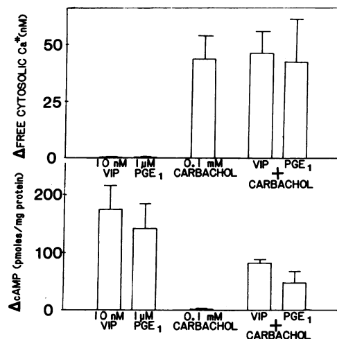
Figure 8. cAMP and free cytosolic \text{Ca}^{2+} in response to carbachol, VIP, and \text{PGE}_1 . cAMP was measured in monolayers similar to those using for Ussing chamber studies using New England Nuclear radioimmunoassay kits, while free cytosolic calcium was measured in dispersed \text{T}_{84} cells as described in Methods. The results are expressed as mean \pm SE of the changes in cAMP or free cytosolic \text{Ca}^{2+} from 3 to 10 monolayers. For \Delta\text{cAMP} , the changes were calculated from the cAMP level 15 min after stimulation by the agents indicated minus the basal cAMP, which was 5 \pm 1 \text{ pmol}/\text{mg} protein. For free cytosolic \text{Ca}^{2+} , the values were calculated as the difference between the basal concentration and the peak concentration after the addition of the agent indicated. The average baseline level of free cytosolic calcium in these five groups was from 112 \pm 12 to 125 \pm 11 \text{ nM} . The increase in free cytosolic \text{Ca}^{2+} induced by carbachol was not altered by VIP or \text{PGE}_1 . Similarly, the increase in cAMP by VIP or \text{PGE}_1 was not altered by carbachol.
