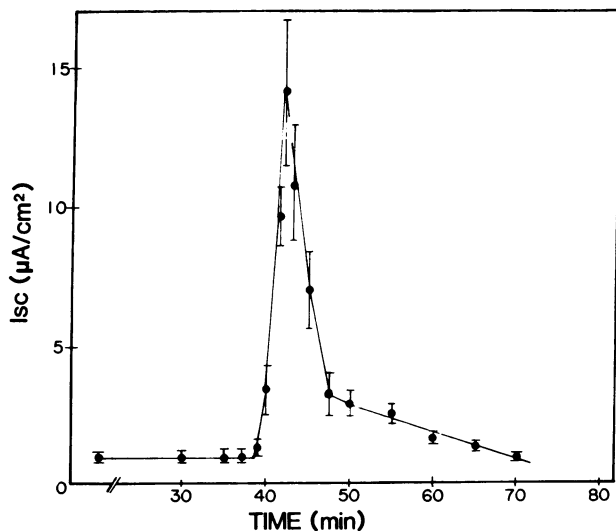
Figure 1. Time-course of the I_{sc} response to 10^{-4} carbachol. Results are expressed as mean \pm SE of six monolayers. Addition of carbachol to the serosal surface resulted in an immediate increase in the I_{sc} , and reached a peak within 5 min. Thereafter, the I_{sc} rapidly declined, but did not reach the baseline until \sim 30 min after the addition.
