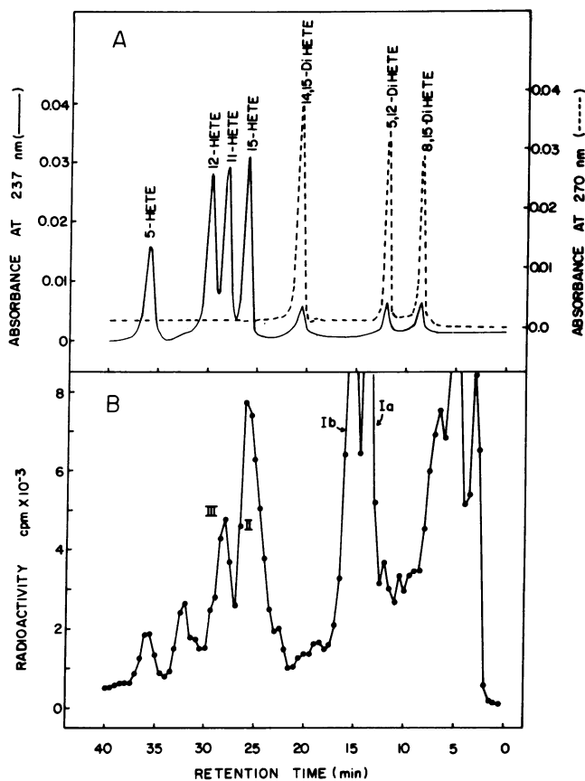
Figure 2. Reverse-phase HPLC of silicic acid column-purified human umbilical arterial HETEs. Intact human umbilical arterial segments (200 mg, dry weight) were incubated with [ 1\text{-}^{14}\text{C} ]arachidonic acid (10 \mu\text{M} ) for 30 min in 10 ml of Tris-Hanks'. Incubation medium was extracted as described. After silicic acid column chromatography, [ 1\text{-}^{14}\text{C} ]HETEs were analyzed by reverse-phase HPLC as described in Methods. Fractions of 0.5 ml were collected, and radioactivity in 0.25-ml aliquots from each fraction was determined by liquid scintillation counting (B). Reference 5-, 11-, 12-, and 15-HETE (monitored at 237 nm) as well as 5,12-, 8,15-, and 14,15-diHETE at 270 nm) were chromatographed under identical HPLC conditions (A).
