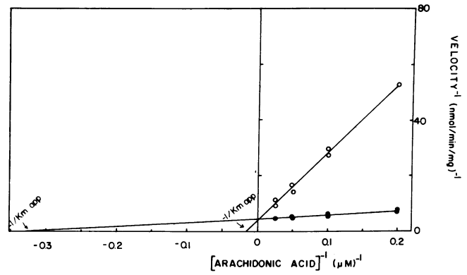
Figure 5. Kinetic analyses of inhibition by 15-HETE of the enzymatic conversion of [ 14 C]arachidonic acid to prostaglandins by cyclooxygenase from human umbilical arterial microsomes. Arterial microsomal protein (400 μg in 500 μl of Tris-GSH) was preincubated in the presence (○) or absence of 15-HETE (100 μM) (●) for 5 min at room temperature. Cyclooxygenase activity was assayed with varying concentrations of [ 14 C]arachidonic acid (5–40 μM) at 37°C for 5 min. Cyclooxygenase activity is expressed as the sum of 6kPGF 1α , PGE 2 , and PGF 2α production (no PGI 2 , TXB 2 , or PGD 2 was detected in these experiments). Lineweaver–Burk plots were generated using linear regression analyses.
