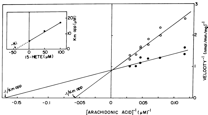
Figure 9. Kinetic analyses of inhibition by 15-HETE of the enzymatic conversion of [ 1\text{-}^{14}\text{C} ]arachidonic acid to prostaglandins by cyclooxygenase from endothelial cell microsomes. Endothelial cell microsomal protein (250 \mu\text{g} in 500 \mu\text{l} of Tris-GSH) was preincubated in the presence ( \circ ) or absence ( \bullet ) of 15-HETE (100 \mu\text{M} ) for 5 min at room temperature. Cyclooxygenase activity was assayed with varying concentrations of [ 1\text{-}^{14}\text{C} ]arachidonic acid (8.6–34.5 \mu\text{M} ) at 37^\circ\text{C} for 5 min. Cyclooxygenase activity is expressed as the sum of 6\text{kPGF}_{1\alpha} , \text{PGE}_2 , \text{TXB}_2 , and \text{PGF}_{2\alpha} production (no \text{PGD}_2 or \text{PGI}_2 was detected in these experiments). Lineweaver-Burk plots were generated using linear regression analyses. (Inset) K_m apparent from experiments at 0, 50, and 100 \mu\text{M} 15-HETE were calculated and K_i determined from linear regression analysis of a Dixon plot.
