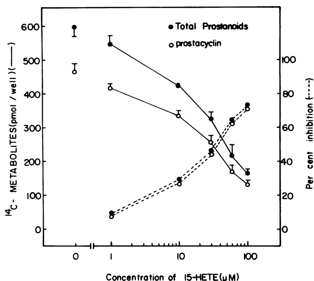
Figure 8. Concentration-dependent inhibition by 15-HETE of the conversion of exogenous [1- 14 C]arachidonic acid to prostaglandins. Fetal bovine aortic endothelial cell monolayers were preincubated for 15 min with the indicated concentrations of 15-HETE (1–100 \mu M), in 750 \mu l of MEM. [1- 14 C]arachidonic (5 \mu M) was then added and the incubation was continued for a further 60 min. The products were extracted in chloroform-methanol as previously described and analyzed by TLC radioautography-liquid scintillation counting. Values represent the mean \pm 1 SD of four different experiments. Total prostacyclin is sum of 6kPGF 1α and PGI 2 production. Total prostanoids are sum of 6kPGF 1α , PGF 2α , PGE 2α , PGI 2 , and TXB 2 production. No PGD 2 was detected in these experiments.
