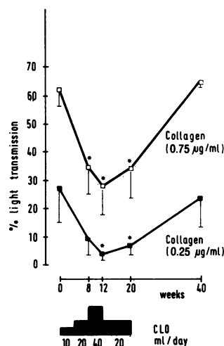
Figure 3. Platelet aggregation on 0.25/0.75 \mu g/ml collagen (% light transmission, mean \pm SEM, n = 6 ) before, during, and after intake of dietary cod liver oil (CLO). *, P < 0.05 , paired t test as compared to time 0.
