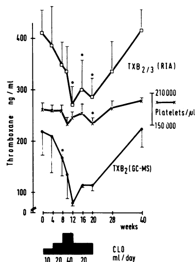
Figure 6. Platelet count (platelets/μl) in blood and thromboxane formation in serum of clotted whole blood (ng/ml, mean±SEM) before, during, and after intake of dietary cod liver oil (CLO) in various dosages. Thromboxane (TX) B 2/3 ( n = 6) was measured radioimmunologically (RIA), thromboxane B 2 ( n = 3) was measured by combined gas chromatography/mass spectrometry (GC-MS). *, P < 0.05, paired t test as compared to time 0.
