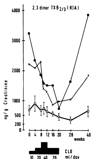
Figure 5. Endogenous thromboxane A 2/3 production as measured by the urinary metabolites 2,3-dinor thromboxane (TX) B 2/3 (ng/g of creatinine, mean±SEM, n = 4) before, during, and after dietary intake of cod liver oil (CLO). The metabolites were measured radioimmunologically (RIA).
