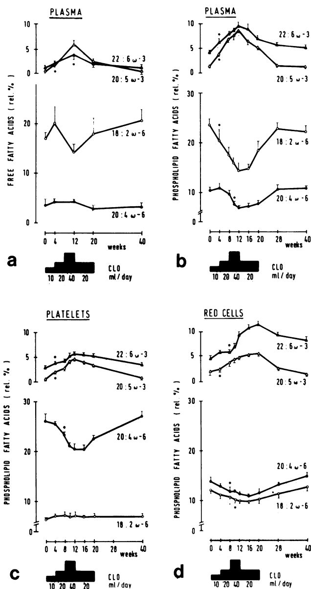
Figure 1. Fatty acids (relative %, mean \pm SEM, n = 6 ) in (a) plasma, (b) plasma phospholipids, (c) platelet phospholipids, and (d) erythrocyte membrane phospholipids before, during, and after ingestion of dietary cod liver oil (CLO) in various dosages. Palmitic, stearic, and oleic acid remained constant throughout the study. *, P < 0.05 , paired t test as compared to time 0.
