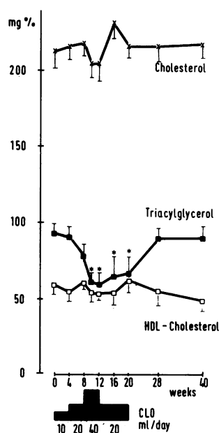
Figure 2. Serum lipids (mg%, mean \pm SEM, n = 6 ) before, during, and after dietary intake of cod liver oil (CLO) at the indicated HDL, high density lipoprotein. *, P < 0.05 , paired t test as compared to time 0.
