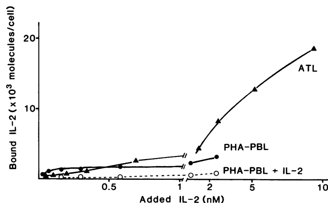
Figure 5. Radiolabeled IL-2 binding to normal peripheral blood lymphocytes cultured in the presence of 0.1% PHA-P for 7 d (PHA-PBL) and to 5-d-cultured ATL leukemic cells obtained from patient M.S. Nonsaturable binding was determined by incubating cells with 250-fold excess amount of unlabeled IL2. Nonsaturable binding curve of only the PHA-P-stimulated cells (PHA-PBL + IL-2) is shown in this figure. Binding curves for ATL leukemic cells (ATL) and PHA-P-stimulated lymphocytes (PHA-PBL) are specific binding curves which were obtained by subtracting unsaturable binding.
