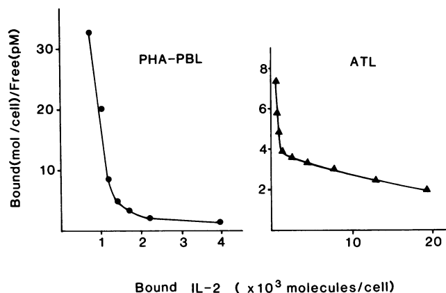
Figure 6. A Scatchard plot of radiolabeled IL-2 binding data shown in Fig. 5. The results indicate that there are two different classes of IL-2 receptors with two different affinities. Calculated high and low affinity receptor numbers are 1,300 and 8,000/cell in PHA-PBL, and 2,100 and 37,500/cell in ATL leukemic cells, respectively. The affinities obtained from Scatchard analysis of both high and low affinity receptors are K_a = 6.9 \times 10^{10} \text{ M}^{-1} , 8.8 \times 10^8 \text{ M}^{-1} in PHA-PBL, and K_a = 1.1 \times 10^{10} \text{ M}^{-1} , 9.5 \times 10^8 \text{ M}^{-1} in ATL leukemic cells, respectively. PHA-PBL, PHA-stimulated lymphocytes.
