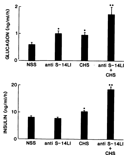
Figure 5. Comparison of the effects of CHS (1 mM) and a sheep somatostatin antibody (anti-S-14 LI) alone and in combination on glucagon and insulin release from monolayer islet cell cultures. Medium glucose concentration, 5.5 mM. NSS = control incubations with nonimmune sheep serum ( n = 5 for each incubation condition) *, P < 0.05 vs. NSS; **, P < 0.01 vs. anti-S-14 LI or CHS.
