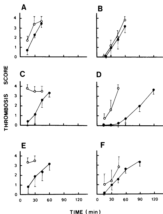
Figure 1. Antithrombotic effect of intact H (A, B) and of h 16 (C, D) and h 12 (E, F) in a venous thrombosis model in rabbits. ○, free heparin moieties; ●, covalent complexes between the heparin moieties and AT. A, C, and E, 55 µg/kg dose; B, D, and F, 110 µg/kg dose. The data represent mean±SD of at least four experiments.
