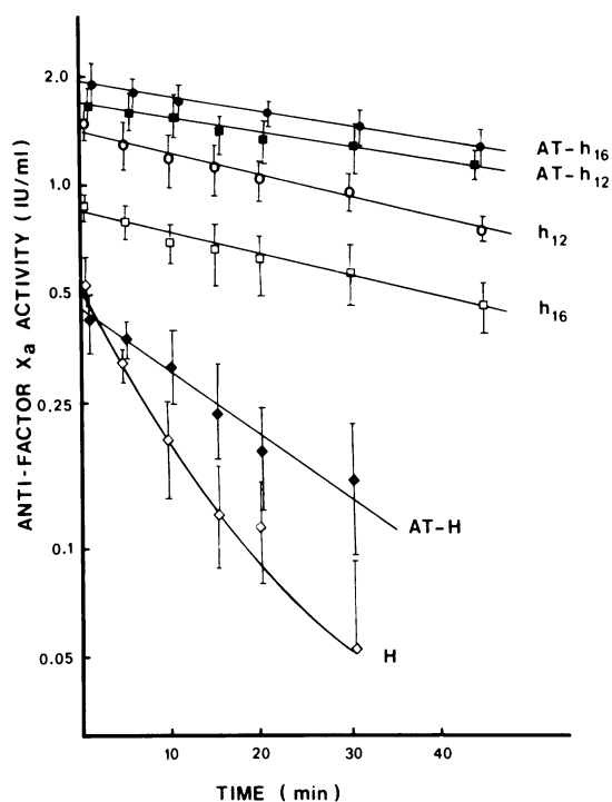
Figure 2. Initial disappearance rate of anti-Factor Xa activity after intravenous injection into rabbits of 110 µg/kg free or complexed heparin moieties.
