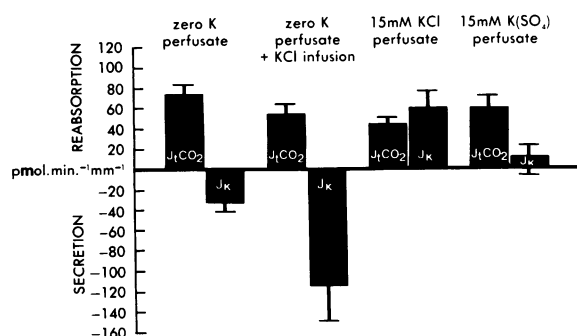
Figure 1. J_{\text{tCO}_2} and J_K values during distal tubule in vivo perfusion in four experimental settings. Shown are mean values±SEM.
