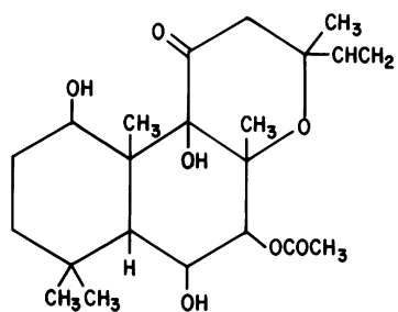
Figure 1. Forskolin.
