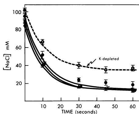
Figure 3. Time course of the continuous change in tubular fluid [NaCl] after intervals of stop-flow in K-depleted, \circ , control, \bullet , K-infused, \blacksquare , and K-repleted, \blacktriangle , rats. The lines were calculated from the equation: C_t = (C_0 - C_{Eq})e^{-\tau t} + C_{Eq} (see Methods). Calculated values of the \tau and the C_{Eq} were taken from Table II. Measured tubular fluid concentrations at steady state and after 10, 30, 45, and 60 s of stop-flow presented in Table I are also plotted on this figure.
