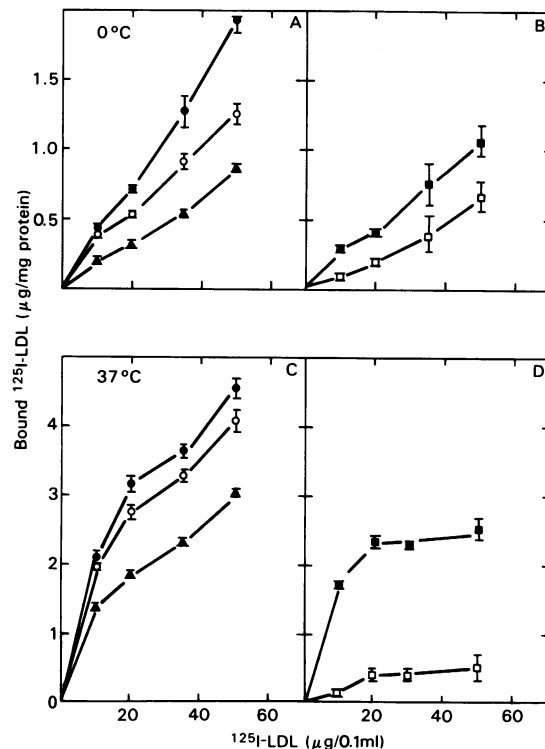
Figure 2. The effect of incubation temperature, calcium, EDTA, and excess unlabeled LDL on the binding of ^{125}\text{I} -LDL to adult human hepatic membranes. From 138 to 182 \mu\text{g} of hepatic membranes were added to a 75 mM NaCl, 150 mM TrisCl buffer containing 1 mM \text{CaCl}_2 (●), 30 mM EDTA (○) or 20-fold excess unlabeled LDL (▲). These mixtures were then incubated for 30 min at the indicated concentrations of ^{125}\text{I} -LDL at either 0°C (A and B) or 37°C (C and D). Total specific binding (■) and EDTA sensitive binding (□) were the differences between the binding observed in the absence and presence of unlabeled LDL and between the binding observed in 1 mM \text{CaCl}_2 and 30 mM EDTA, respectively. Values represent the mean \pm SE of triplicate samples.
