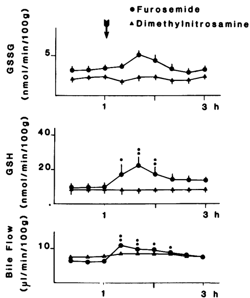
Figure 9. Biliary excretion of GSSG and GSH after the administration of furosemide ( n = 5 ) and dimethylnitrosamine ( n = 3 ), two compounds generating electrophilic metabolites that do not deplete hepatic GSH. Mean \pm SE. GSSG is expressed as GSH equivalents. ** P < 0.01 * P < 0.05 .
