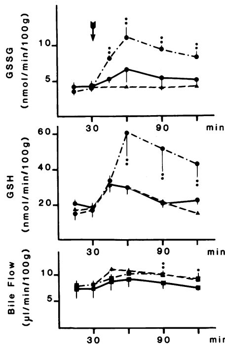
Figure 6. Effect of aminopyrine ( \bullet ), 80 \mu\text{mol}/100 \text{ g i.p.} (dotted line) and 8 \mu\text{mol}/100 \text{ g i.p.} (solid line) and 8 \mu\text{mol}/100 \text{ g i.p.} ( \blacktriangle ) of ethylmorphine on the biliary excretion of GSH. Aminopyrine increased the biliary excretion of GSSG slightly but the GSSG/GSH ratio did not change because of the proportional increase in the efflux of GSH. Mean \pm SE of five rats. GSSG is expressed as GSH equivalents; **, P < 0.01 ; *, P < 0.05 .
