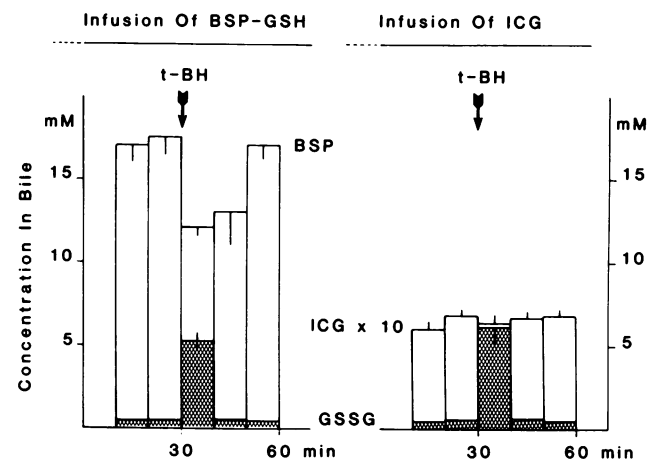
Figure 4. During a constant infusion of BSP-GSH at a rate of 540 nmol/min per 100 g the intraperitoneal administration of 1.4 mmol/kg of t -butyl hydroperoxide ( t -BH) produced a significantly smaller increase in the biliary concentration of GSSG (hatched bars) than in the control rats shown in Fig. 3 ( n = 7 ). Moreover, the increase in biliary GSSG produced by the hydroperoxide led to a significant decrease in the biliary concentration of BSP-GSH (open bars). In contrast, during a constant infusion (25 nmol/min per 100 g) of indocyanine green, which is not conjugated with GSH and is transported by a separate carrier, the maximal biliary concentration of the dye did not change under identical experimental conditions (mean \pm SE, n = 4 ).
