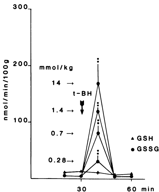
Figure 3. Biliary excretion of GSSG and GSH after the intraperitoneal administration of 0.28–14 mmol/kg of t -butyl hydroperoxide ( t -BH) to rats with a biliary fistula. The hydroperoxide resulted in a dose-dependent increase in the biliary excretion of GSSG, whereas the excretion of GSH remained constant (only highest dose data plotted). Mean \pm SE of six rats; GSSG is expressed as GSH equivalents; **, P < 0.01 .
