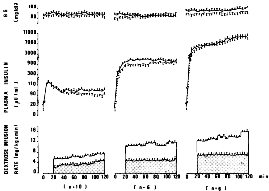
FIGURE 1 Euglycemic clamp. Plasma glucose (BG), plasma insulin, and dextrose infusion rate (mean±SEM) during euglycemic clamp at ~100, ~1,000, and ~10,000 \mu\text{U}/\text{ml} plasma insulin concentration, after placebo (—, □) or 7-d prednisone (15 plus 15 mg/d) (- - -, □).
