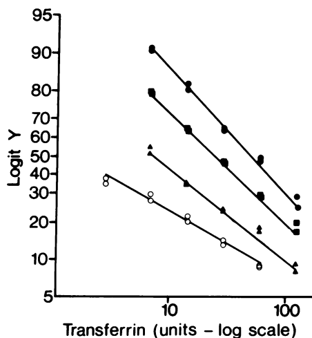
FIGURE 10 Parallel line assays of serial dilutions of rat serum (○ — ○); duodenal cell homogenate (● — ●); ileal cell homogenate (■ — ■); and mixture of serum and duodenal cell homogenate (▲ — ▲). The F test for homogeneity of variance and the Student's t test showed a significant difference ( P < 0.001 ) in the slopes of the serum and intestinal transferrins (method of Rodbard and Lewald [24]). The transferrin is in arbitrary units. The ordinate is logit Y (In Y/1-Y) where Y is bound count/uninhibited count rate).
