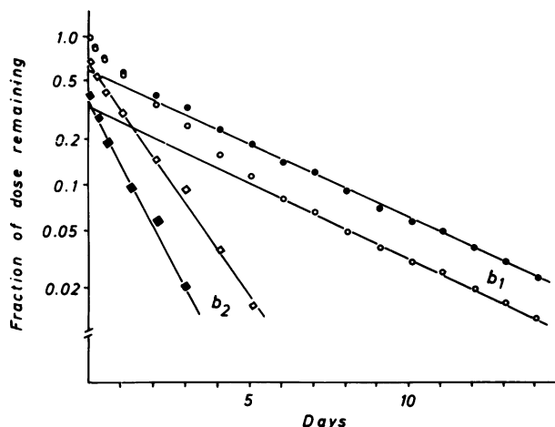
FIGURE 1 Serum die-away curves of subject 1 (Table II) after intravenous injection of ^{125}\text{I} -Lp(a) (●) and ^{131}\text{I} -LDL (○). The fraction of injected radioactivity remaining in the serum is plotted semilogarithmically against time. The radioactivity decay curves can be resolved into two exponential components. The first exponential ( b_1 ) was calculated from the terminal linear portion of the decay curve. The second exponential [ b_2 for Lp(a) ♦, b_2 for LDL ◇] was obtained by subtraction of the first exponential from the serum die-away curve.
