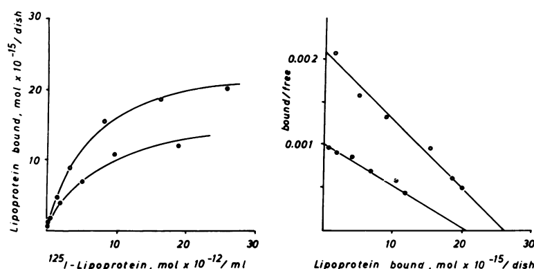
FIGURE 2 125 I-Lp(a) and 125 I-LDL binding to fibroblast monolayers as a function of lipoprotein concentration. Fibroblast monolayers (340 μg protein/dish) were incubated with increasing concentrations (1–100 μg/ml) of 125 I-Lp(a) (●) or 125 I-LDL (○) at 4°C for 2 h. Left panel: The amount of lipoprotein bound specifically to surface receptors is plotted against the lipoprotein concentration in the medium. The specific binding refers to the difference in binding under the two conditions described in the method section. Each value represents the mean of two or three determinations in a typical experiment. Right panel: Scatchard plots of 125 I-Lp(a) (●) and 125 I-LDL (○) binding. The data from the left panel have been replotted. The linear regression analysis bound/free vs. bound yielded intercepts on the abscissa (maximal binding capacity) of 20.94 × 10 -15 mol/dish for Lp(a) and of 25.91 × 10 -15 mol/dish for LDL. The equilibrium dissociation constants, estimated from the slopes of the regression lines, were 9.32 × 10 -9 M for Lp(a) and 5.65 × 10 -9 M for LDL.
