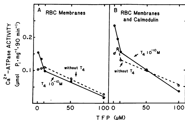
FIGURE 2 The effect of TFP on \text{Ca}^{2+} -ATPase activity in erythrocyte membranes, with and without added T 4 and calmodulin. The enzyme assay was carried out as described in Methods, in the presence or absence of T 4 , 10 -10 M. Panels A and B show enzyme activity in the absence and presence, respectively, of calmodulin, 100 ng/mg membrane protein per ml assay volume. TFP concentrations were 0, 5, 10, 50, and 100 \mu\text{M} . The data represent the mean values of enzyme activity in duplicate samples from three experiments.
