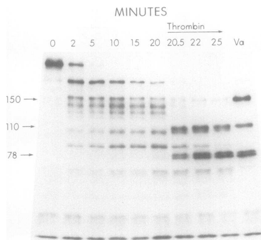
FIGURE 3 Proteolysis of ^{125}\text{I} -labeled Factor V by a sonicated platelet suspension. Platelets at a concentration of 10^8/\text{ml} in a buffer containing 0.15 M NaCl, 20 mM Tris-HCl pH 7.4, 2.5 mM \text{CaCl}_2 , 5.5 mM glucose, and 5 mg/ml recrystallized bovine serum albumin were disrupted by sonicating twice for 15 s at 25 W at 4^\circ\text{C} . The suspension was then equilibrated to 22^\circ\text{C} and Factor V ( 5\text{ }\mu\text{g}/\text{ml} , 1,500 cpm/ng) was added. At the indicated times samples were taken and mixed with an equal volume of buffer containing sodium dodecyl sulfate and 5% 2-mercaptoethanol and then boiled for 2 min. Samples containing 30 ng of ^{125}\text{I} -labeled protein were electrophoresed on a 7.5% polyacrylamide slab gel containing sodium dodecyl sulfate with a 4% stacking gel according to Laemmli (21). Protein was detected by autoradiography (22). At 20 min 2 U/ml of thrombin was added to the reaction mixture.
