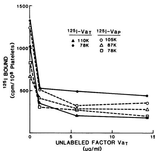
FIGURE 6 Binding of ^{125}\text{I-Va}_T and ^{125}\text{I-V}_{ap} to platelets and displacement by \text{Va}_T (Methods). ^{125}\text{I-V}_{aT} and ^{125}\text{I-V}_{ap} were derived from 100 ng/ml of ^{125}\text{I-V} (2,405 cpm/ng).
