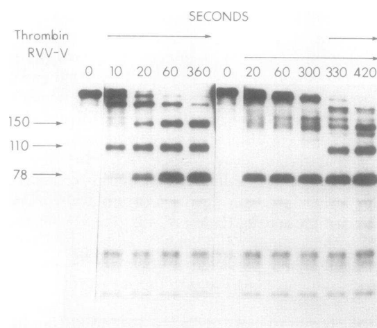
FIGURE 1 Activation of ^{125}\text{I} -labeled Factor V by thrombin and RVV-V. ^{125}\text{I} -labeled Factor V (5 \mu\text{g}/\text{ml} 214 cpm/ng) in a buffer containing 0.5 M NaCl, 20 mM Tris, pH 7.4, 2.5 mM CaCl 2 , 5.5 mM glucose, recrystallized and bovine serum albumin, 5 mg/ml at 22°C, was treated with thrombin (0.2 U/ml) or RVV-V (20 \mu\text{g}/\text{ml} ). After 300 s thrombin (0.2 U/ml) was added to the sample that was treated with RVV-V. At the indicated times samples were taken, mixed with an equal volume of buffer containing sodium dodecyl sulfate and 5% 2-mercaptoethanol, and boiled for 2 min. Samples containing 30 ng of ^{125}\text{I} -labeled protein were then electrophoresed on a 7.5% polyacrylamide slab gel containing sodium dodecyl sulfate with a 4% stacking gel according to Laemmli (21). Protein was detected by autoradiography (22).
