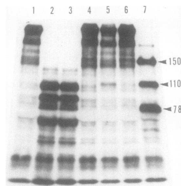
FIGURE 4 Requirements for the expression of the Factor V activator in human platelets. ^{125}\text{I} -Factor V ( 5\text{ }\mu\text{g}/\text{ml} , 1,300 cpm/ng) was incubated in a buffer containing 0.15 M NaCl, 20 mM Tris-HCl pH 7.4, 2.5 mM \text{CaCl}_2 , 5.5 mM glucose, and recrystallized bovine serum albumin, 5 mg/ml at 22^\circ\text{C} for 20 min in the presence of the following additional components (a) None. (b) Frozen and thawed platelets 3 \times 10^9/\text{ml} . (c) Frozen and thawed platelets 3 \times 10^9/\text{ml} , 93\text{ }\mu\text{M} DAPA. (d) Intact platelets 3 \times 10^9/\text{ml} . (e) 2 U/ml thrombin and 93\text{ }\mu\text{M} DAPA. (f) Platelets at a concentration of 3 \times 10^9/\text{ml} pretreated with thrombin for 5 min followed by addition of 93\text{ }\mu\text{M} DAPA and then the Factor V. After a 20-min incubation samples were taken and dissolved in an equal volume of buffer containing sodium dodecyl sulfate and 5% 2-mercaptoethanol and boiled for 2 min. Samples containing 30 ng of ^{125}\text{I} -labeled protein were electrophoresed on a 7.5% polyacrylamide slab gel containing sodium dodecyl sulfate with a 4% stacking gel according to Laemmli (21). Protein was detected by autoradiography (22).
