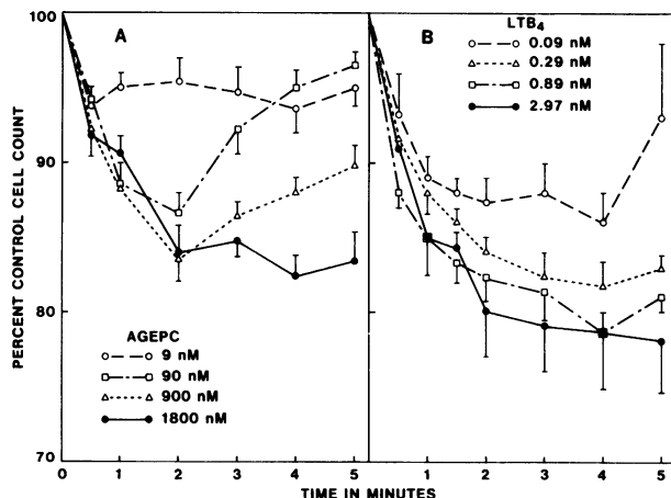
FIGURE 1 Concentration-dependent stimulation of human neutrophil aggregation by AGEPC and \text{LTB}_4 . Human neutrophils ( 2.5 \times 10^6 cells/ml) were incubated for 5 min at 37^\circ\text{C} , and then challenged with either from 9 to 1800 nM AGEPC or from 0.09 to 2.97 nM \text{LTB}_4 . At 0.5, 1.0, 2.0, 3.0, 4.0, and 5.0 min after the addition of agonist, cell counts were determined and compared with the control (pre-agonist) cell count. Data are presented as the mean \pm SEM of four (AGEPC) or five ( \text{LTB}_4 ) separate experiments. The fall in cell count represents aggregation of the neutrophils.
