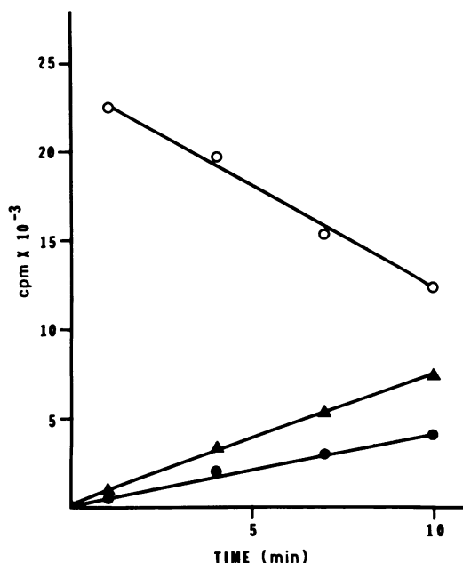
FIGURE 4 Bilirubin UDP-glucuronyltransferase activity in microsomes of human small intestine. Incubations were carried out with [ 14 C]bilirubin (5.22 mCi/mol; 4.6 \mu M) as substrate and 0.67 mg microsomal protein per assay. At the indicated time points, incubations were terminated by addition of methanol and carrier pigment in the form of rat bile. Bilirubin glucuronides were converted to their corresponding mono- and dimethylesters, extracted, and quantitated as described in Methods. Results are expressed as radioactivity (counts per minute) recovered after thin-layer chromatography. The data represent a typical result. O, [ 14 C]UCB; \blacktriangle , [ 14 C]BMG; \bullet , [ 14 C]BDG.
