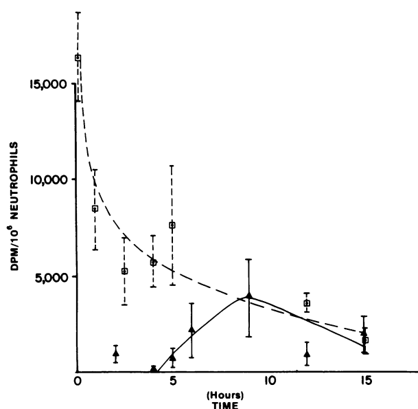
FIGURE 4 Neutrophil specific activity. Specific activity of lung ( \Delta ) and blood ( \square ) neutrophils in rabbits after the infusion of ^{111}\text{In} -labeled peritoneal neutrophils. (Bars indicate standard errors).
