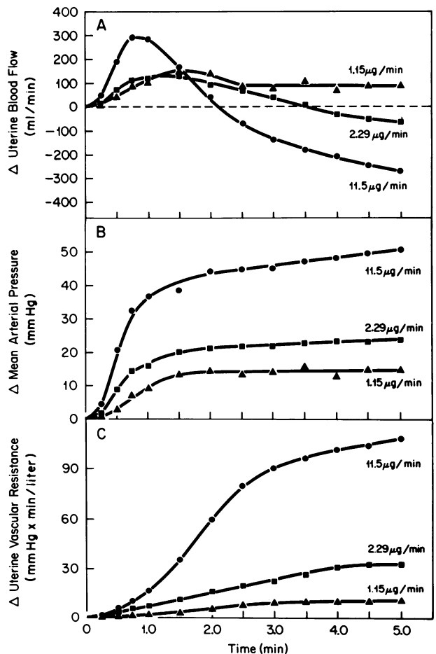
FIGURE 5 The simultaneous changes in UBF (A), MAP (B), and UVR (C) during the continuous systemic infusion of [\text{Val}^5] ANG II. The data for three doses are presented. Each point represents the mean value for seven experiments.
