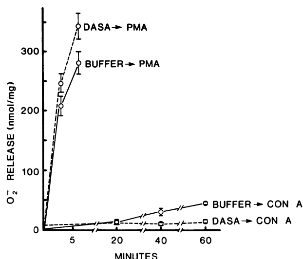
FIGURE 1 Effect of DASA pretreatment on \text{O}_2^- release by neutrophils stimulated with PMA or Con A, plotted as a function of time. Neutrophils were exposed to DASA in buffer (KRP-D) or to buffer alone, washed, then assayed for \text{O}_2^- production in the presence of either PMA (10 ng/ml) or Con A (100 \mu\text{g}/\text{ml} ). The values plotted for each stimulus are the means; the bars represent the SEM. The means of three experiments performed in triplicate with Con A as stimulus are shown; the number of experiments (in triplicate) in the presence of PMA was four at 0 min, eleven at 3 min, and 9 at 6 min. Inhibition by DASA with Con A as stimulus was significant at 40 min ( P = 0.025 ) and 60 min ( P = 0.006 ), using paired values in Student's t test.
