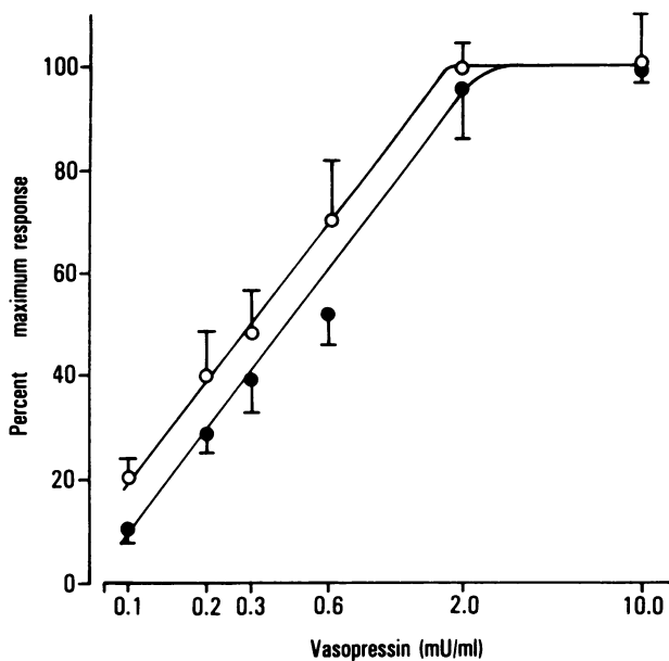
FIGURE 4. Effects of U46619 on vasopressin-stimulated water flow. Hemibladders were pretreated with indomethacin (50 \mu M) for 1 h. Vasopressin (●) or vasopressin plus U46619 (1 \mu M) (○) was added to the serosal baths and water flow was measured for 30 min. After thorough washing to return water flow to basal levels and a 30-min recovery period, a supra-maximal dose of vasopressin (10 mU/ml) or vasopressin plus U46619 (1 \mu M) was added and water flow was determined for another 30 min. Water flow is expressed as a percentage of this maximum response ( 64.3 \pm 4.6 mg/min per 10 cm 2 , n = 72 ). Each point represents the mean \pm SEM for six hemibladders. U46619 significantly ( P < 0.001 ) increased vasopressin-stimulated water flow and significantly shifted the dose-response curve to the left ( P < 0.001 ) in a parallel fashion (slopes were 0.64 for the control hemibladders and 0.62 for the U46619-treated hemibladders).
