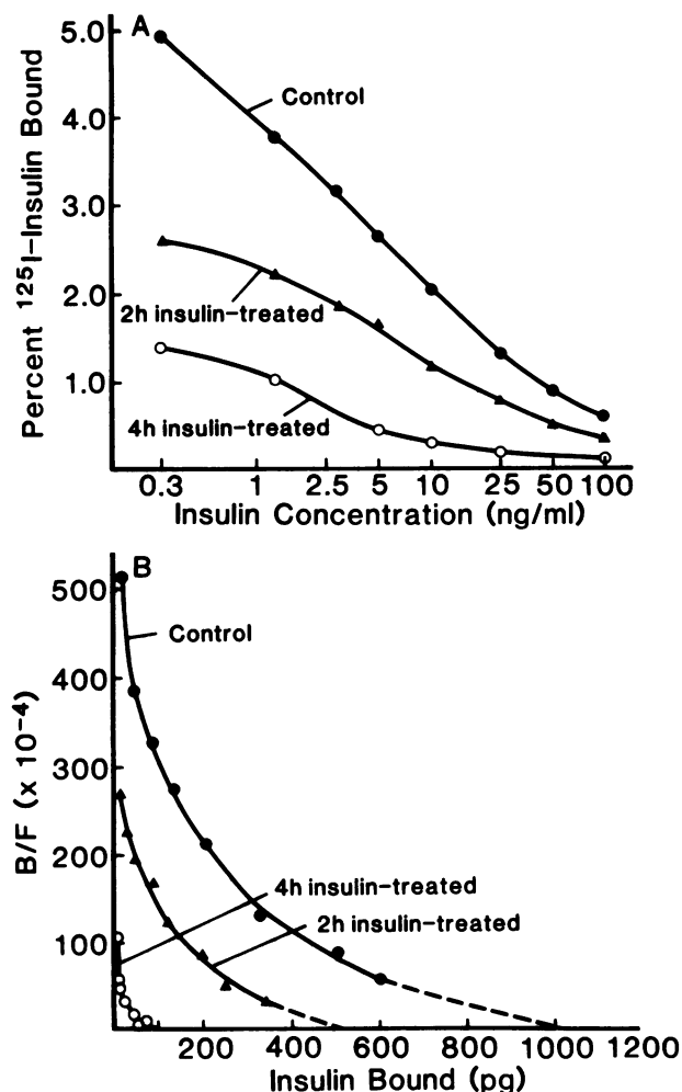
FIGURE 2 Ability of 2- and 4-h insulin-treated adipocytes to specifically bind ^{125}\text{I} -insulin at various insulin concentrations. A Adipocytes ( 2.5 \times 10^6 ) were preincubated either in the absence of insulin ( \bullet ) or in the presence of 100 ng/ml insulin for either 2 h ( \blacktriangle ) or 4 h ( \circ ) at 37^\circ\text{C} , and prebound insulin dissociated as previously described. Cells were then incubated for 3 h at 16^\circ\text{C} with 0.3 ng/ml ^{125}\text{I} -insulin, plus unlabeled insulin, to give the indicated total insulin concentrations. All data are corrected for nonspecific binding. B Scatchard plots of these insulin binding data for control ( \bullet ), 2 h ( \blacktriangle ), or 4 h ( \circ ) insulin-treated cells. The ratio of bound to free insulin ( B/F ) is plotted on the ordinate, and bound insulin on the abscissa.
