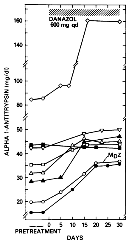
FIGURE 1 Effect of danazol administration on serum \alpha 1-antitrypsin levels in the eight study patients (R.J., ●; D.K., ○; H.P., ▲; T.W., △; M.G., ■; L.E., □; E.M., ▽; A.J., ◇). All individuals were type PiZ except D.K. (PiM D Z) and A.J. (PiSZ).
