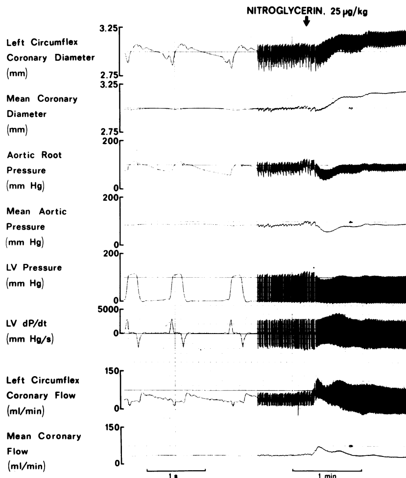
FIGURE 4 The effects of a bolus of nitroglycerin, 25 \mu\text{g/kg} , in a conscious dog are depicted on simultaneous and continuous measurements of phasic and mean left circumflex coronary artery diameter, aortic root pressure, left ventricular pressure, left ventricular dP/dt , and phasic and mean left circumflex coronary blood flow. Nitroglycerin induced a transient fall in coronary diameters and a striking early increase in coronary blood flow. However, coronary diameters then rose as all other measured variables returned to control levels. The marked sinus arrhythmia is characteristic of the conscious dog.
