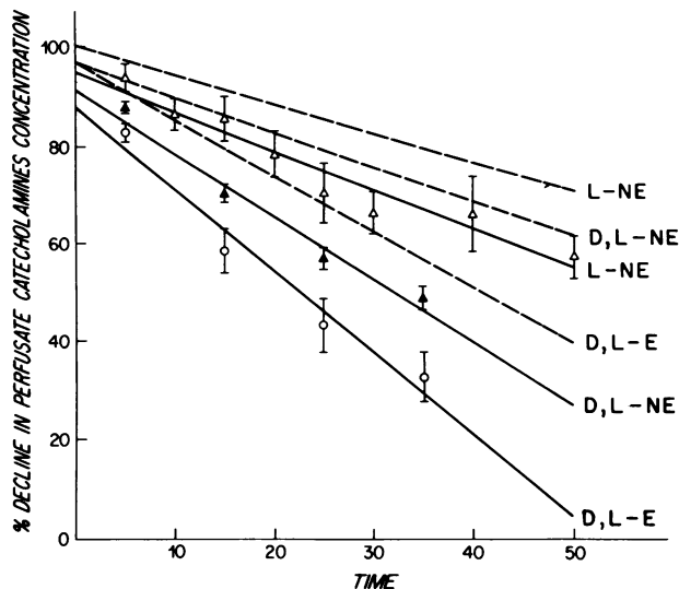
FIGURE 3 Rate of disappearance of [ 3 H]catecholamines from the perfusion medium. Time (minutes) is on the horizontal axis; on the vertical axis is the concentration at various times after the addition of [ 3 H]catecholamine as a function of the initial concentration. Values are means \pm SEM plotted according to the method of least squares. Note that the fall is monoexponential with a t_{1/2} of 26 min for E and 60 min for NE. The dotted lines represent the theoretical rate of disappearance for NE and E if total catecholamine clearance resulted from excretion in urine. The predicted t_{1/2} for NE is 85 min and for E, 43 min.
