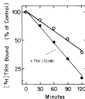
FIGURE 1 Reversibility of [ ^3\text{H} ]TRH binding. Identical samples of cells from a single culture were incubated with 25 nM [ ^3\text{H} ]TRH. After 90 min (zero time) the cells were washed, resuspended in fresh medium with 25 nM [ ^3\text{H} ]TRH (control cells), with no added TRH (0), or with 10 nM unlabeled TRH (■) and the amount of [ ^3\text{H} ]TRH bound measured at the times indicated. Control cells bound 0.60 pmol [ ^3\text{H} ]TRH per milligram protein. The points represent the mean of duplicate values whose average variation was \pm 13\% .
