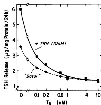
FIGURE 5 Effect of T_3 on basal and TRH-stimulated TSH release. Equal aliquots of cells were incubated with medium alone or T_3 , 0.1 to 10 nM. After 48 h the cells were centrifuged, resuspended in fresh medium and divided equally into four tubes. Two tubes were incubated in medium alone (basal) and two tubes in 10 nM TRH for an additional 24 h after which TSH release was measured. Average cell protein was 42 \mu g/tube . Points represent the mean of duplicate determinations whose mean SD was \pm 10\% .
