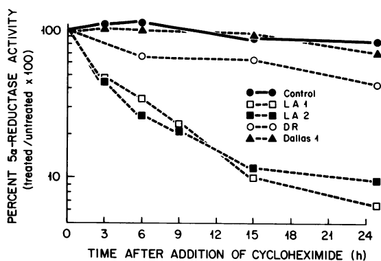
FIGURE 6 Stability of 5 \alpha -reductase in intact cells. Cells were grown in small Linbro plates as described in the text. On day 7 cycloheximide was added to half the wells of each cell strain to make the final concentration 1 mM. 5 \alpha -Reductase activity was assayed using the whole cell at 0, 3, 6, 9, 15, and 25 h after the addition of cycloheximide. The control strain was 188. LA, Los Angeles; DR, Dominican Republic.
