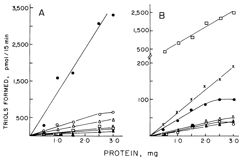
FIGURE 3 Effect of enzyme concentration on hydroxylation of 5\beta -[G- ^3 H]cholestane- 3\alpha , 7\alpha -diol by human liver mitochondria (A) and microsomes (B). Standard assay conditions were employed, except for protein concentration. \square — \square , 5\beta -cholestane- 3\alpha , 7\alpha ,12 \alpha -triol; \blacktriangle — \blacktriangle , 5\beta -cholestane- 3\alpha , 7\alpha ,24-triol (24R); \triangle — \triangle , 5\beta -cholestane- 3\alpha , 7\alpha ,24-triol (24S); \times — \times , 5\beta -cholestane- 3\alpha , 7\alpha ,25-triol; \bullet — \bullet , 5\beta -cholestane- 3\alpha , 7\alpha ,26-triol (25R), and \circ — \circ , 5\beta -cholestane- 3\alpha , 7\alpha ,26-triol (25S).
