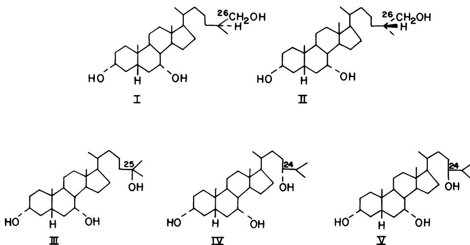
FIGURE 1 Structures of 5\beta -cholestanetriols: I, 5\beta -cholestane- 3\alpha,7\alpha,26 -triol (25R); II, 5\beta -cholestane- 3\alpha,7\alpha,26 -triol (25S); III, 5\beta -cholestane- 3\alpha,7\alpha,25 -triol; IV, 5\beta -cholestane- 3\alpha,7\alpha,24 -triol (24R); and V, 5\beta -cholestane- 3\alpha,7\alpha,24 -triol (24S).
