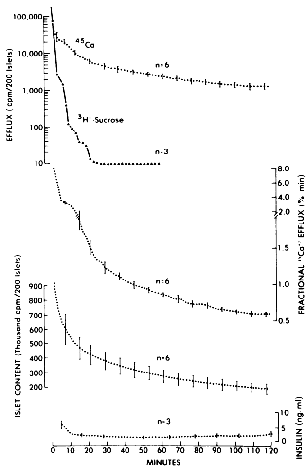
FIGURE 1 Efflux of ^{45}\text{Ca} from prelabeled rat islets. [^3\text{H}]\text{Sucrose} was used as a marker for the extracellular space. Basal perfusate contained 2.2 mM glucose and 0.05 mM \text{Ca}^{+2} . Fractional ^{45}\text{Ca} efflux was calculated at 2-min intervals as explained in Methods. Data shown as mean \pm SEM.
