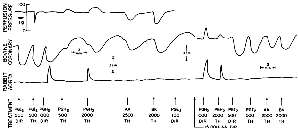
FIGURE 7 Comparison of the effect of PGI 2 and PGH 2 on the isolated perfused rabbit heart. The PGI 2 was stored in an ethanol stock. The ethanol was evaporated in a stream of N 2 and was diluted as a 50-mM Tris buffer pH 9 solution just before use. The PGH 2 was stored as an acetone stock solution. The organic solvent was removed in a stream of N 2 and redissolved in a 50-mM phosphate buffer (pH 7.4) just before use. The number below each agonist indicates the amount in nanograms injected. DIR-denotes direct application of standards to the assay tissues, and TH-denotes injections through the heart. The 15-hydroperoxy-arachidonic acid (15 · OOH · AA) was dissolved in 0.1 M Tris pH 7.4 buffer and was infused over the assay tissues at a final concentration of 1 μg/ml for 15 min before testing.
