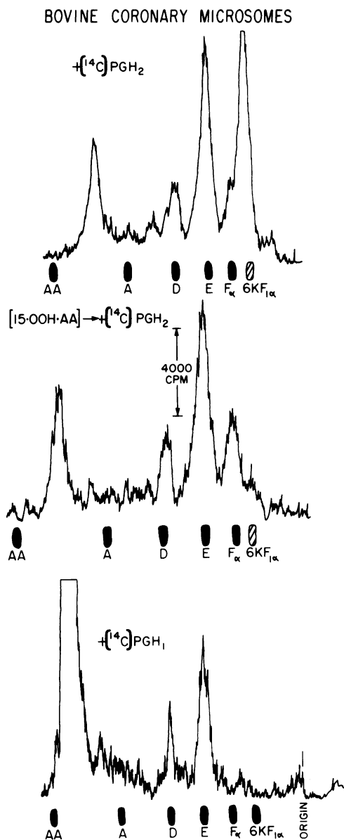
FIGURE 6 The enzymatic generation of PGI 2 . Bovine coronary microsomes (10 mg protein) were incubated in a 100-mM phosphate buffer, pH 7.9, with 25 μg of [ 14 C]PG endoperoxide (60,000 cpm) for 20 min at 37°C. The reaction mixture was acidified to pH 3.5 and extracted twice with ethyl acetate; concentrated and separated on a silica gel G plate in the A-9 solvent system. Note that the 6-keto-PGF 1α (6KF 1α ) runs just before the PGF 2α standard. There is no 6-keto-PGF 1α formed with microsomes that were preincubated with 15-hydroperoxy-arachidonic acid (15 · OOH · AA), a known in vitro antagonist of PGI 2 synthesis or when microsomes are incubated with [ 14 C]PGH 1 .
