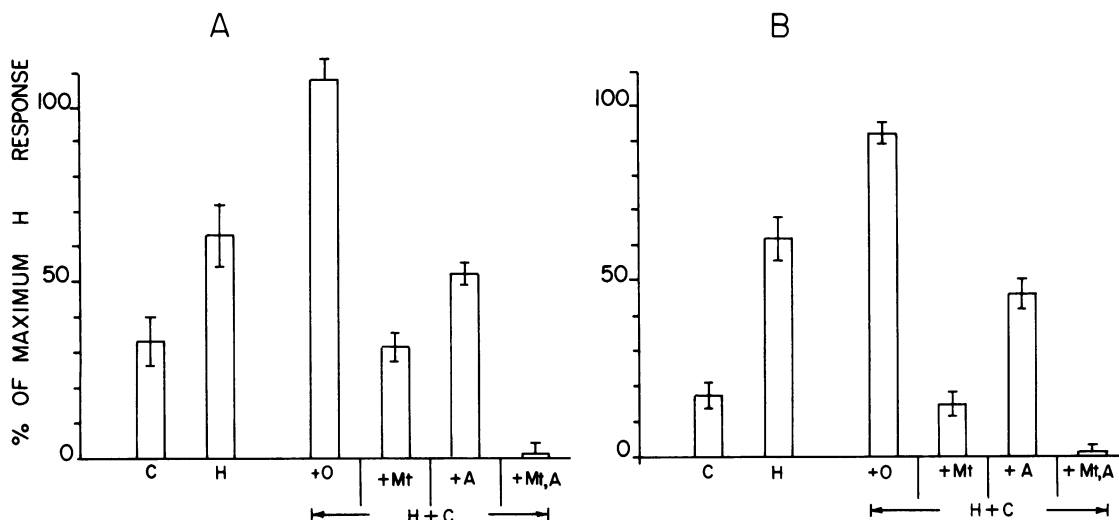
FIGURE 5 The effects of metiamide (Mt) and atropine (A) on the histamine-carbamylcholine interaction. Oxygen uptake is expressed as the percentage of the maximal response above basal produced by histamine (H) ( 10 \mu\text{M} ). (A) The data represent the mean \pm SE based upon four determinations from a single preparation of cells. The agents were studied at the following concentrations: 10 \mu\text{M} carbamylcholine (C), 1 \mu\text{M} histamine, 10 \mu\text{M} metiamide, and 10 \mu\text{M} atropine. (B) The data represent the mean \pm SE based upon six determinations pooled from two separate preparations of cells with the same agents as in A except for the use of 1 \mu\text{M} carbamylcholine. The response to 10 \mu\text{M} histamine was 73.3% above basal in A and 89.8 and 92.5% above basal in the two experiments in B. 0.1 \text{ mM} IMX was present in all incubations where histamine was studied.
