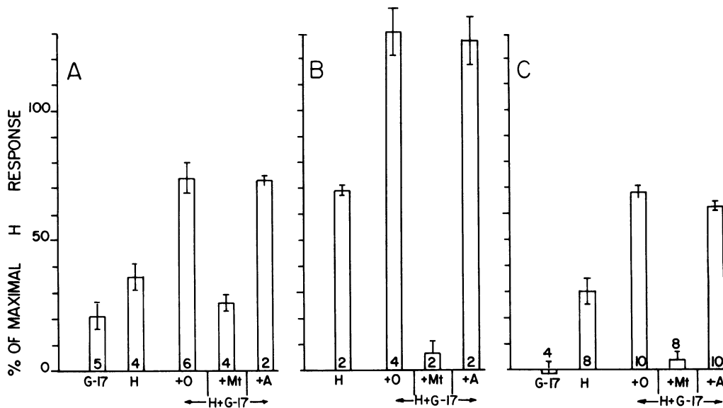
FIGURE 3 The effects of metiamide (Mt) and atropine (A) on the histamine-gastrin interaction. Oxygen uptake was determined for unenriched mucosal cells and expressed as the percentage of the maximal increment above basal produced by histamine (H) (10 \mu M). Each panel represents a separate preparation, with the data representing the mean \pm SE for the indicated number of determinations. The following concentration of agents were used: 0.1 \mu M heptadecapeptide gastrin (G-17), 0.1 mM IMX, 10 \mu M metiamide, 10 \mu M atropine, 0.1 \mu M histamine in panels A and C, and 1 \mu M histamine in panel B. The maximal responses produced by 10 \mu M histamine were 98.6%, 50.1% and 75.9% above basal in panels A, B, and C, respectively. 0.1 mM IMX was present in all incubations where histamine was used.
