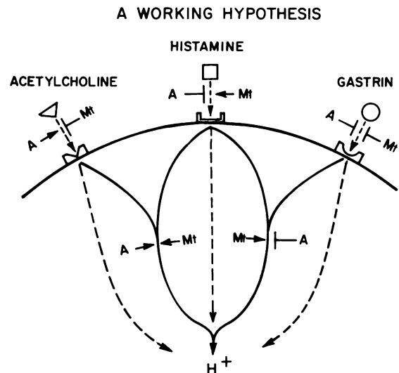
FIGURE 6 A working model for the actions and interactions of secretagogues on the isolated parietal cell. The dashed lines represent independent actions of secretagogues, and the solid lines represent interactions. Sites at which atropine (A) and metiamide (Mt) are respectively inhibitory (→) and at which these agents are not inhibitory (—) are indicated.
