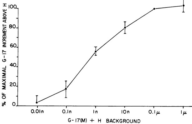
FIGURE 2 The dose-response relationship to gastrin with a histamine (H) background. The dose-response relationship for heptadecapeptide gastrin (G-17) was tested with a histamine background of 1 \mu\text{M} in one preparation and 0.1 \mu\text{M} in two others. The data represent the mean \pm SE (based upon preparation means) for at least duplicate determinations in each preparation and have been expressed as the percentage of the maximal increment above the histamine background produced by the addition of 0.1 \mu\text{M} G-17. This concentration of gastrin produced a maximal response in two of the three preparations. In these experiments 0.1 \mu\text{M} histamine produced responses 14.0 and 17.6% above basal. The addition of G-17 (0.1 \mu\text{M} ) produced responses that were, respectively, 57.8 and 46.4% above basal. The 1 \mu\text{M} histamine background produced a response that was 38.2% above basal and the addition of 0.1 \mu\text{M} G-17 resulted in a response 92.3% above basal. 0.1 mM IMX was present for all incubations with histamine.
