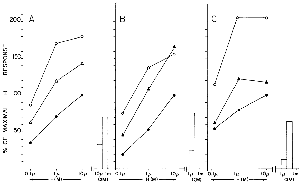
FIGURE 4 The effects of carbamylcholine (C) on the dose-response relationship to histamine (H). Oxygen uptake was determined in three separate preparations and represents the mean of at least duplicate determinations in each preparation and has been expressed as the percentage of the maximal increment above basal produced by histamine ( 10 \mu\text{M} ). Histamine ( \bullet ) was also tested with the following agents as background: 1 \text{ mM} carbamylcholine ( \circ ), 10 \mu\text{M} carbamylcholine ( \Delta ) and 1 \mu\text{M} carbamylcholine ( \blacktriangle ). The responses to carbamylcholine alone are indicated by the open bars. The maximal responses to histamine ( 10 \mu\text{M} ) were 69.7%, 36.5%, and 83.8% above basal in panels A, B, and C, respectively. 0.1 \text{ mM} IMX was present when histamine was used.
