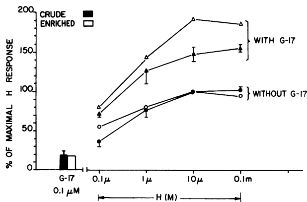
FIGURE 1 The effect of gastrin on the dose-response relationship for histamine (H). Oxygen uptake is expressed as the percentage of the maximal increment above basal produced by 10 \mu\text{M} histamine. The responses to histamine ( \bullet ), histamine plus 0.1 \mu\text{M} heptadecapeptide gastrin (G-17) ( \blacktriangle ), and 0.1 \mu\text{M} G-17 alone (closed bar) were studied in three separate preparations of unenriched cells and in a single enriched preparation with 53% parietal cells (histamine, \circ ; histamine plus 0.1 \mu\text{M} G-17, \Delta ; and 0.1 \mu\text{M} G-17 alone, open bar). In the separate preparations each point represents at least duplicate independent determinations. Error bars represent SE, based upon preparation means. 10 \mu\text{M} histamine produced a mean response of 89.7 \pm 7.6\% above basal in the preparations of unenriched cells and 42.3\% above basal with the enriched cells. 0.1 \text{ mM} IMX was present when histamine was used.
