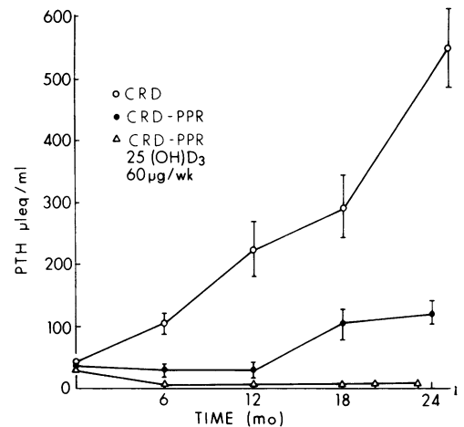
FIGURE 3 Representation of mean \pm SE for serum PTH levels as a function of time in the three groups of dogs. Group I ( \circ — \circ ) consisted of the four dogs with CRD ingesting 1,200 mg P/day; Group II, as defined in the text ( \bullet — \bullet ), includes the four dogs with CRD maintained on proportional reduction of P (PRP); Group III ( \triangle — \triangle ) includes the six dogs with CRD on the proportional reduction regimen plus supplemental 20 \mu\text{g} of 25(\text{OH})\text{D}_3 three times per week.
