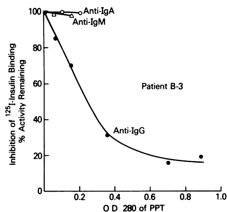
FIGURE 9 Effect of specific immunoprecipitation on binding-inhibitory activity of serum B-3. 200- \mu l samples of serum B-3 were incubated with various amounts of anti-human immunoglobulin antisera of indicated specificity in a final volume of 500 \mu l. Incubation and assay were carried out as described in the legend to Fig. 8.
