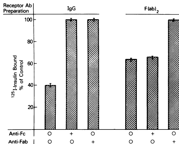
FIGURE 7 Effect of IgG and F(ab) 2 fractions of IgG on ^{125} I-insulin binding to IM-9 lymphocytes. (left) 100 \mu l of DEAE peak 1 (obtained as in legend to Fig. 1) was incubated in duplicate with 100 \mu l of anti-human IgG directed at the Fc or the Fab portion of the molecule, or with PBS alone. After 1 h at 37°C, the immune precipitates were sedimented in a Beckman Microfuge, and duplicate 50- \mu l samples of the supernate were assayed for inhibition of insulin binding. Assay tubes contained 5 \times 10^6 IM-9 lymphocytes, 100 pg of ^{125} I-insulin, and 50 \mu l of the above supernates or PBS alone, with a final volume of 700 \mu l/tube. One set of tubes contained, in addition, 10 \mu g/ml of unlabeled insulin. The assay was completed and data were calculated as in the legend to Fig. 2. (right) An F(ab) 2 fraction of IgG was prepared as described in Methods. 50- \mu l samples were incubated in duplicate with 100 \mu l of anti-human IgG with specificity for the F(ab) 2 or Fc regions, or with PBS alone for 1 h at 37°C. Immune precipitates were sedimented, and duplicate 50- \mu l samples of the supernatants were assayed for inhibition of insulin binding as described above.
