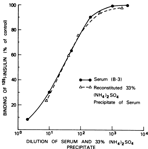
FIGURE 3 Effect of whole serum and 33% ammonium sulfate precipitate of serum on ^{125} I-insulin binding to IM-9 lymphocytes. 2 ml of serum B-3 was precipitated by 33% ammonium sulfate, as described in the Methods, resuspended in 2 ml of PBS, and dialyzed against 200 vol of PBS at 4°C. 3 \times 10^6 IM-9 lymphocytes were then incubated for 60 min at 4°C in 0.4 ml of assay buffer with final dilutions of whole serum or reconstituted 33% ammonium sulfate precipitate as indicated. Cells were then washed three times in 1 ml of PBS at 4°C, after which an insulin-binding assay was performed as in legend to Fig. 2.
