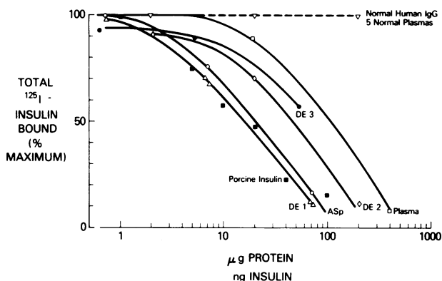
FIGURE 6 Inhibition of ^{125} I-insulin binding by various serum preparations. 5 \times 10^6 IM-9 lymphocytes were incubated with 100 pg of ^{125} I-insulin in a total volume of 0.5 ml of assay buffer, in the presence of increasing amounts of several preparations of serum B-2, normal IgG, or porcine insulin. The preparations included whole plasma, 33% ammonium sulfate precipitate (ASp), DEAE peaks 1, 2, and 3, and porcine insulin. After 90 min at 15°C, duplicate 200- \mu l samples were centrifuged through 100 \mu l of cold buffer, the supernats were aspirated, and ^{125} I-insulin bound to the pellets was determined. Percent of maximal binding was calculated as: (% bound to cells in presence of serum preparation or insulin)/(% bound to cells in presence of buffer alone).
