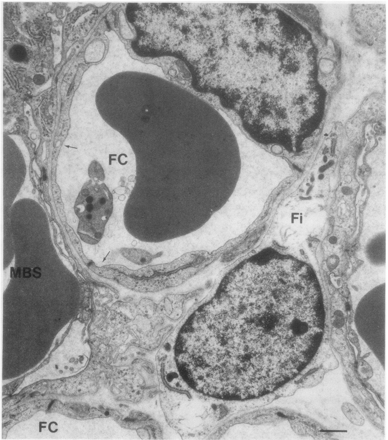
FIGURE 3 Rabbit placenta; a typical epithelial plate on the left side of the central fetal capillary is delineated by arrows. FC, fetal capillary; MBS, maternal blood space; Fi, fibroblast. The three-layered nature of the barrier (endothelium, cytotrophoblast, and syncytiotrophoblast) is clearly visible. The bar is 1 \mu m long.
