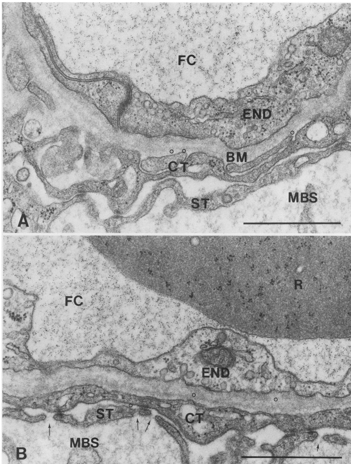
FIGURE 6 Ferritin injections into the fetal circulation. Ferritin particles in the basement membrane (BM) have been circled. A shows an endothelial cell junction, common in epithelial plates. B shows a great abundance of ferritin-filled vesicles in the endothelium (END), some seemingly arranged in chains, and a fetal reticulocyte (R). Both figures show the invaginations in the cytotrophoblast (CT), and B shows the pores (arrows) in the syncytiotrophoblast (ST). Basement membrane matrix material may partially fill the endothelial junctions. Bars are 1 \mu m.
