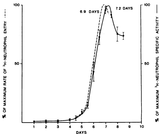
FIGURE 3 Blood appearance time of ^3\text{H} -tdr labeled neutrophils. The solid line was drawn through points representing ^3\text{H} -tdr neutrophil activity in circulation (mean \pm SE of eight determinations). The interrupted line represents the rate of entry of ^3\text{H} -tdr labeled neutrophils and was drawn by correcting each observed point for simultaneous egress of labeled cells from circulation as described in Methods.
