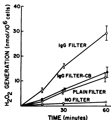
FIGURE 1 Generation of \text{H}_2\text{O}_2 by PMNs contacting non-phagocytosable surfaces, plotted as a function of the length of incubation. 2.5 \times 10^6 PMNs were used, and triplicate reaction mixtures were studied. The means of averaged values are plotted for six experiments; the bars above and below each point represent the SEM. "CB" indicates that the cells were treated with cytochalasin B. Results with IgG-coated filters were significantly greater than those achieved with plain filters or no filters, whether rate ( P < 0.001 ) or peak values ( P < 0.001 ) were analyzed (Duncan's multiple-range test [20]). With IgG-coated filters, cytochalasin B treatment reduced peak \text{H}_2\text{O}_2 generation by 54% ( P < 0.001 ).
