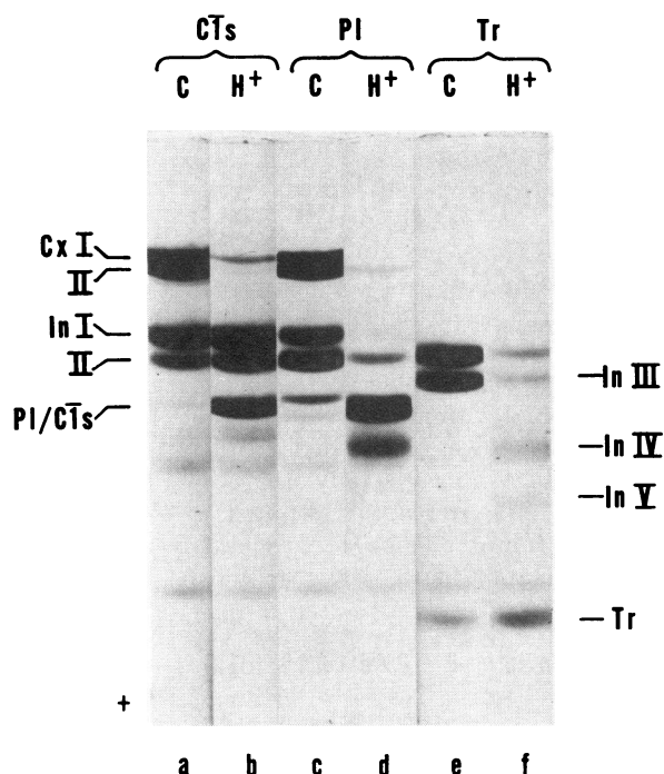
FIGURE 8 SDS gel (5% acrylamide) electrophoretic analysis of the interaction of acid-treated C \bar{1} inactivator with C \bar{1} s, plasmin (PI), and trypsin (Tr). C \bar{1} inactivator (5 mg/ml) was acidified to pH 2.0 with equal volumes of 1/6 N HCl for 30 min at 37°C and neutralized with 1/6 N NaOH. The untreated (C) and acid-treated (H + ) inhibitors (1.5 mg/ml) were then incubated with C \bar{1} s (0.9 mg/ml), plasmin (1.1 mg/ml), or trypsin (320 \mu g/ml) for 10 min at 37°C. The mixtures were analyzed after the addition of an SDS-urea solution. The native C \bar{1} inactivator with buffer, plasmin, or trypsin was applied to gels a, c, and e; and the denatured inhibitor with buffer or the enzymes to gels b, d, and f. "In III" indicates the 86,000 dalton C \bar{1} inactivator trypsin derivative. "In IV" and "In V" indicate the new C \bar{1} inactivator proteolytic derivatives resulting from the action of plasmin (IV) and trypsin (IV, V) on the acid-treated inhibitor (gels d and f). The gels were overloaded with sample in order to render the bands in gel f visible at comparable protein concentrations.
