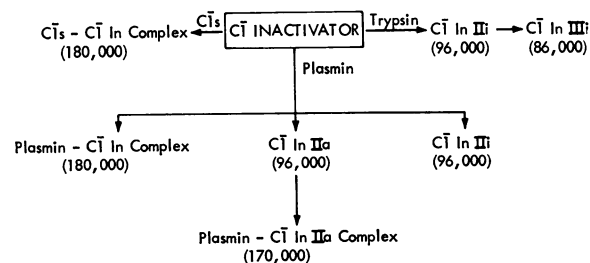
FIGURE 9 Schematic representation of the interactions between C \bar{1} inactivator (C \bar{1} In) and C \bar{1} s, plasmin, and trypsin. The explanation for the nomenclature used is found in footnote 5. The apparent molecular weights of the complexes and of the C \bar{1} inactivator derivatives are indicated in parentheses.
