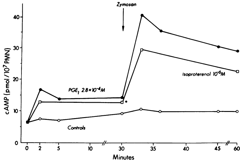
FIGURE 5 Stimulation of cAMP in suspensions of Hypaque/Ficoll-purified human PMN. PMN ( 10^7 ) incubated at 37^\circ\text{C} with 5 \mu\text{g/ml} CB plus 5 \times 10^{-4} M theophylline and with or without (controls) PGE 1 or isoproterenol and then exposed to zymosan. Each point represents the mean of three experiments. (*) Cells were incubated 30 min with PGE 1 and 15 min with isoproterenol before their exposure to zymosan.
