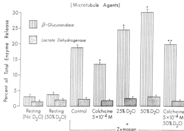
FIGURE 7 Lysosomal enzyme release from CB-treated cells. Human leukocytes ( 4 \times 10^6 ) incubated 10 min with 5 \mu\text{g/ml} CB, incubated 60 min with or without colchicine in appropriate buffer ( \pm\text{D}_2\text{O} ), and exposed to zymosan 30 min. Total (100%) activity (released by 0.2% Triton X-100) for \beta -glucuronidase = 22.8 \pm 2.1 \mu\text{g} phenolphthalein/h/4 × 10^6 cells. Total activity LDH = 462 \pm 51 \text{ AU/4} \times 10^6 cells. (*) Significant at P < 0.01 vs. control. (**) Significant at P < 0.01 vs. 50% D 2 O.
