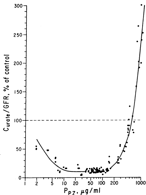
FIGURE 2 C_{urate}/GFR (expressed as percent of control) plotted as a function of P_{Pz} . Each point represents a single clearance period. A few points in the area of greatest density have been omitted. This figure includes 26 experiments.
