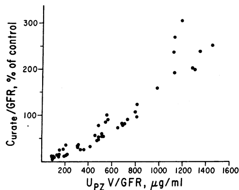
FIGURE 3 C_{urate}/GFR (expressed as percent of control) as a function of pyrazinoate excretion per ml of GFR. Only those data corresponding to P_{Pz} > 100 \mu\text{g/ml} are included (cf. Fig. 2). Each point represents an individual clearance period. The data are from 12 experiments.
