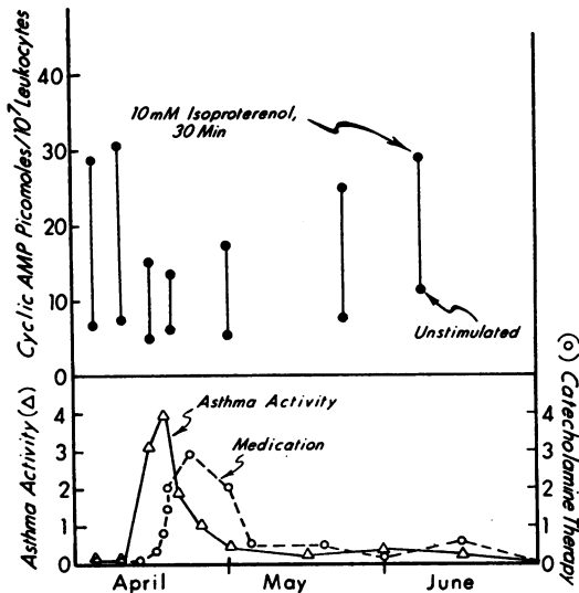
FIGURE 6 Serial mixed leukocyte studies in L. G., a 23 yr old Negro male with pollen allergy, just before, during, and after a sustained period of asthmatic symptoms. The upper closed circles are cyclic AMP values obtained with 10 mM isoproterenol, 37°, 30 min; the lower closed circles are values for unstimulated cells. The lower section of the figure gives the relative severity of asthmatic symptoms and signs (open triangles) and the relative 24 h catecholamine dosage (open circles). In order to compare these responses with the mean isoproterenol response in normal control cells see Table I. At the time of the initial three determinations he had received no therapy. Subsequently he was treated with oral bronchodilator tablets (maximal dose, 4 Tedral tablets/day). During active asthmatic symptoms (> 3 in the figure) the mean FEV 1 was 45% of the predicted vital capacity (two determinations) and the mean duration of forced expiration, 6.2 s. The corresponding values during symptom-free intervals were: FEV 1 93% (the average of single determinations in early April and late May); and mean duration of forced expiration 2.7 s.
