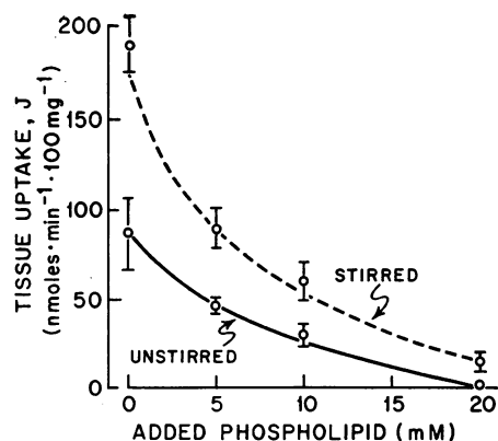
FIGURE 7 Effect of micelle expansion on taurodeoxycholate uptake across the jejunal brush border. Sacs were incubated in buffer containing 20 mM taurodeoxycholate- ^3 H and phospholipid (lecithin) at concentrations of 0, 5, 10, and 20 mM. Uptake rates, J , were determined under unstirred and vigorously stirred (magnetic bar) conditions. Mean values \pm 1 SEM for six determinations at each phospholipid concentrations are shown by the vertical bars.
