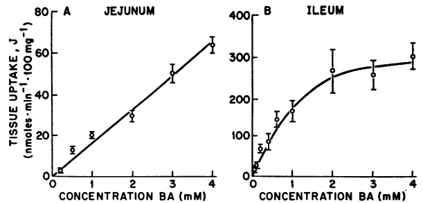
FIGURE 1 Characteristics of bile acid (BA) uptake into the mucosa of the jejunum and ileum. Sacs prepared from jejunum and ileum were incubated in Krebs bicarbonate buffer containing taurocholate- 3 H at concentrations ranging from 0.05–4.0 mM. Mean values ± 1 SEM for 6 to 30 determinations at each concentration are shown by the vertical bars.
