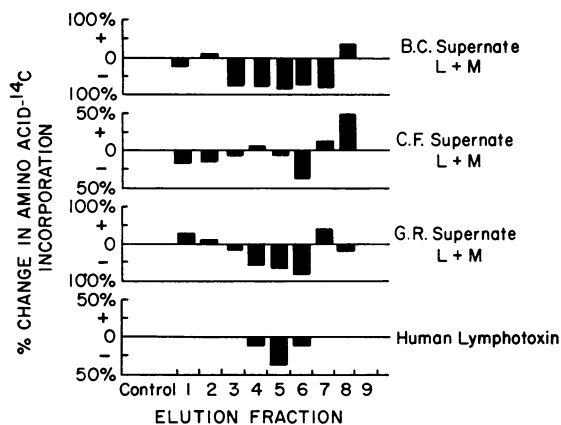
FIGURE 3 Cytotoxicity of eluted fractions of toxic supernates from polymyositis patients compared with that of purified lymphotoxin.
