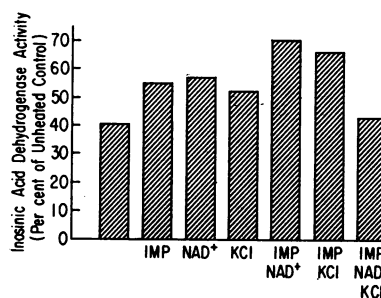
FIGURE 2 Effect of substrates for inosinic acid dehydrogenase on inactivation of the partially purified enzyme at 70^\circ\text{C} for 8 min; IMP, 1.5 \times 10^{-4} M; \text{NAD}^+ , 1.0 \times 10^{-3} M; and KCl, 1 \times 10^{-1} M.
