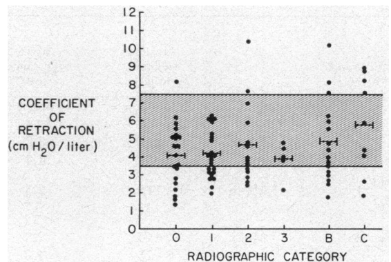
FIGURE 4 Coefficient of retraction in subjects (group 1A and group 2) with different radiographic categories of CWP. (Hatched area represents normal range.)
