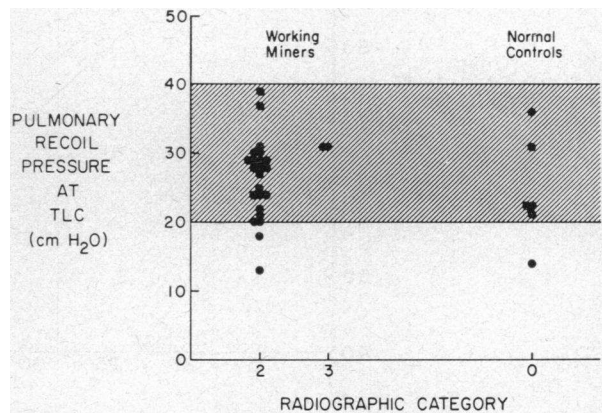
FIGURE 6 Pulmonary recoil pressure at total lung capacity in working miners with categories 2 and 3 (group 1B) and also in normal controls.
