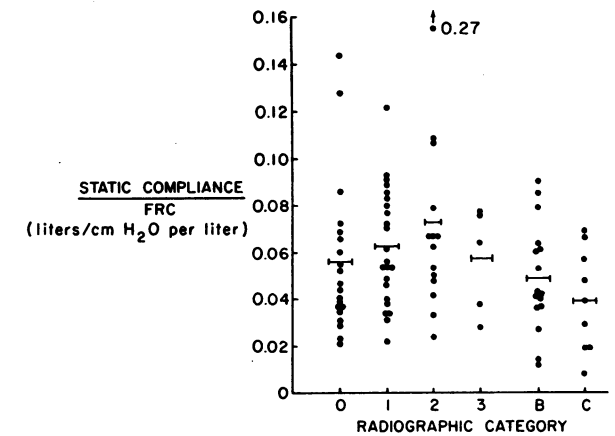
FIGURE 3 Specific compliance in subjects (group 1A and group 2) with different radiographic categories of CWP.
