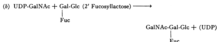
FIGURE 1 Summary of reactions used in the assay of glycosyltransferases. Abbreviations used are: UDP-GalNAc, UDP- N -acetyl- \beta -galactosamine; UDP-Gal, UDP- \beta -galactose; GDP-Fuc, GDP-L-fucose; Gal, \beta -galactose; Glc, \beta -glucose; and Fuc, L-fucose.
