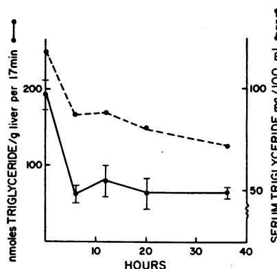
FIGURE 3 The effect of CPIB on glycerol- ^{14}\text{C} incorporation into hepatic triglyceride and on serum triglyceride after 6-36 hr of feeding. Values recorded are means for four rats at each time period. The SE is indicated for triglyceride formation. All differences from control rats are significant ( P < 0.01 ).
