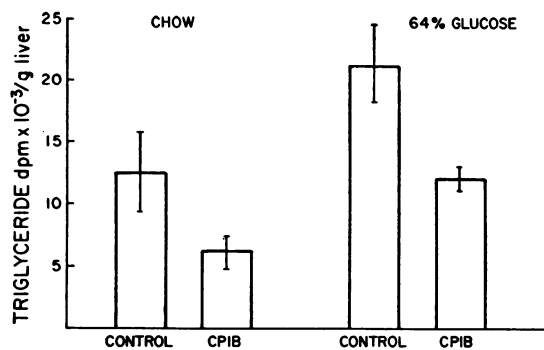
FIGURE 2 Triglyceride synthesis in animals given CPIB. Eight animals in each of the four groups were fed the appropriate diet for 2 wk. Glycerol- ^{14}\text{C} incorporation into hepatic triglyceride in the CPIB treated rats was significantly less than the corresponding control in both diet groups ( P < 0.025 ). Incorporation into triglyceride was significantly increased in animals fed 64% glucose compared with those fed laboratory chow with or without addition of CPIB ( P < 0.05 ). The hepatic triglyceride concentration was 10.3 \pm 1.1 mg/g in rats fed 64% glucose and this increased to 14.9 \pm 2.1 mg/g in those fed the same diet plus CPIB for 14 days.
