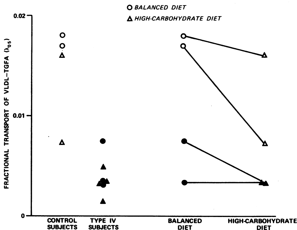
FIGURE 6 Comparison of fractional transport of VLDL-TGFA ( \lambda_{05} ) in control subjects (open symbols) and type IV subjects (closed symbols) on balanced diet (circles) and on high-carbohydrate diet (triangles). At the right are shown the shifts in the four paired studies induced by the high-carbohydrate diet.
