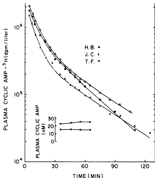
FIGURE 3 Plasma cyclic AMP- 3 H disappearance curves following single rapid intravenous injection of the tracer in man. Time is expressed in relation to the time of injection ( t=0 ). The experimental points are plotted on semilogarithmic coordinates, and the curves were obtained by least squares fits using a digital computer. The plasma levels of endogenous cyclic AMP are plotted in the insets (note Cartesian coordinates) for J. C. and T. F.; a single pooled plasma sample representing the same four points was obtained for H. B.
