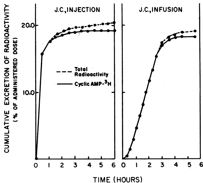
FIGURE 4 Cumulative urinary excretion of cyclic AMP- 3 H (solid lines) and total radioactivity (broken lines) following cyclic AMP- 3 H injection (left panel) and infusion (right panel), subject J. C. Time is expressed in relation to t=0 , the time of tracer injection or infusion initiation. Cumulative excretion is expressed as per cent of administered dose of cyclic AMP- 3 H. The cumulative cyclic AMP- 3 H excretion predicted from the relative magnitudes of plasma clearance rate and renal clearance was 19.5% for the injection study (Table V) and 18.6% for the infusion study (Table IV).
