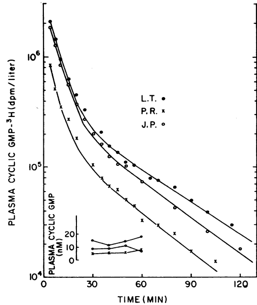
FIGURE 5 Plasma cyclic GMP- ^3\text{H} disappearance curves following single rapid intravenous injection of the tracer in man. Time is expressed in relation to the time of injection ( t=0 ). The experimental points are plotted on semi-logarithmic coordinates, and the curves were obtained by least squares fits using a digital computer. The plasma levels of endogenous cyclic GMP are plotted in the insets (note Cartesian coordinates).
