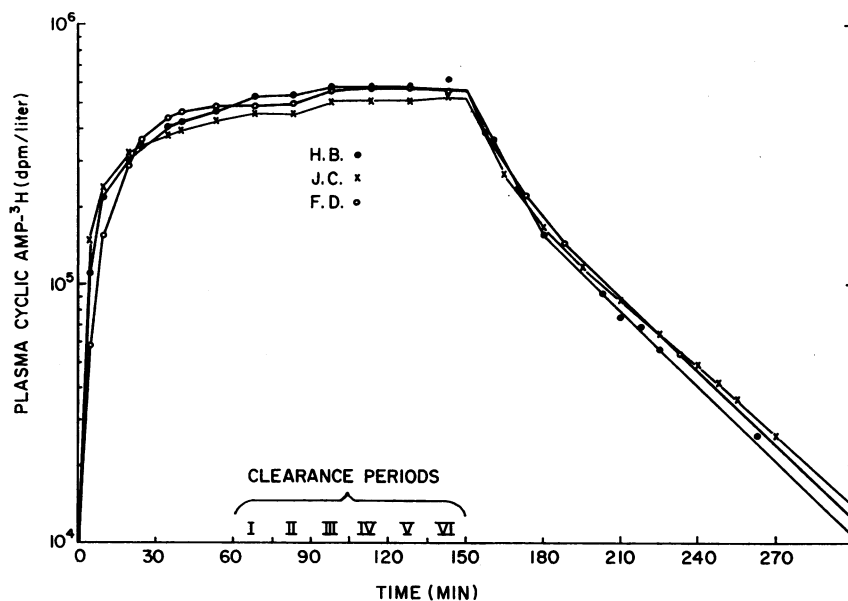
FIGURE 1 Plasma cyclic AMP- 3 H appearance and disappearance curves during and following constant intravenous infusion of the tracer in man. Note the semilogarithmic plot. Time is expressed in relation to infusion initiation ( t=0 ); the infusions were terminated at 150 min. The roman numerals I-VI along the abscissa signify the six successive 15-min clearance periods obtained in each study. Plasma samples for endogenous cyclic AMP determination were drawn at 98, 113, 128, and 143 min.
