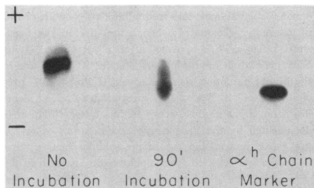
FIGURE 3 Formation of free \alpha^{\text{hem}} -chains from \alpha_2^{\text{hem}}\beta_2^{\text{o}} at 50°C. Starch-gel electrophoresis at pH 8.6; amido black stain. Incubation for 90 min (middle channel) produces a heterogeneous mixture with components exhibiting slower anodal migration than unincubated \alpha_2^{\text{hem}}\beta_2^{\text{o}} (left channel), one identical with marker free \alpha^{\text{hem}} -chains used as a marker (right channel).
