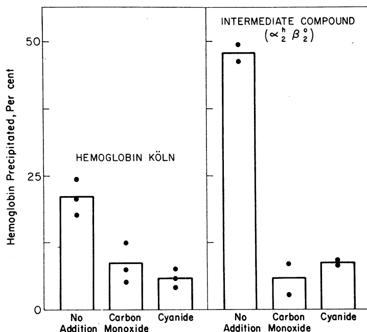
FIGURE 2 Inhibition of heat precipitation of hemoglobin Köln (left) and \alpha_2^{\text{hem}}\beta_2^{\text{o}} (right) by cyanide or carbon monoxide. Both heme-proteins copiously precipitate when heated at 50°C for 2 hr unless the heme ligands, cyanide or carbon monoxide, are present.
